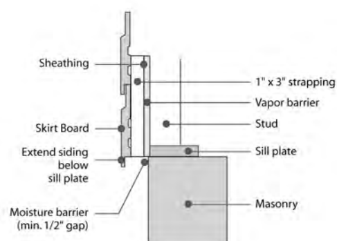
Skirt board - Installation on masonry
